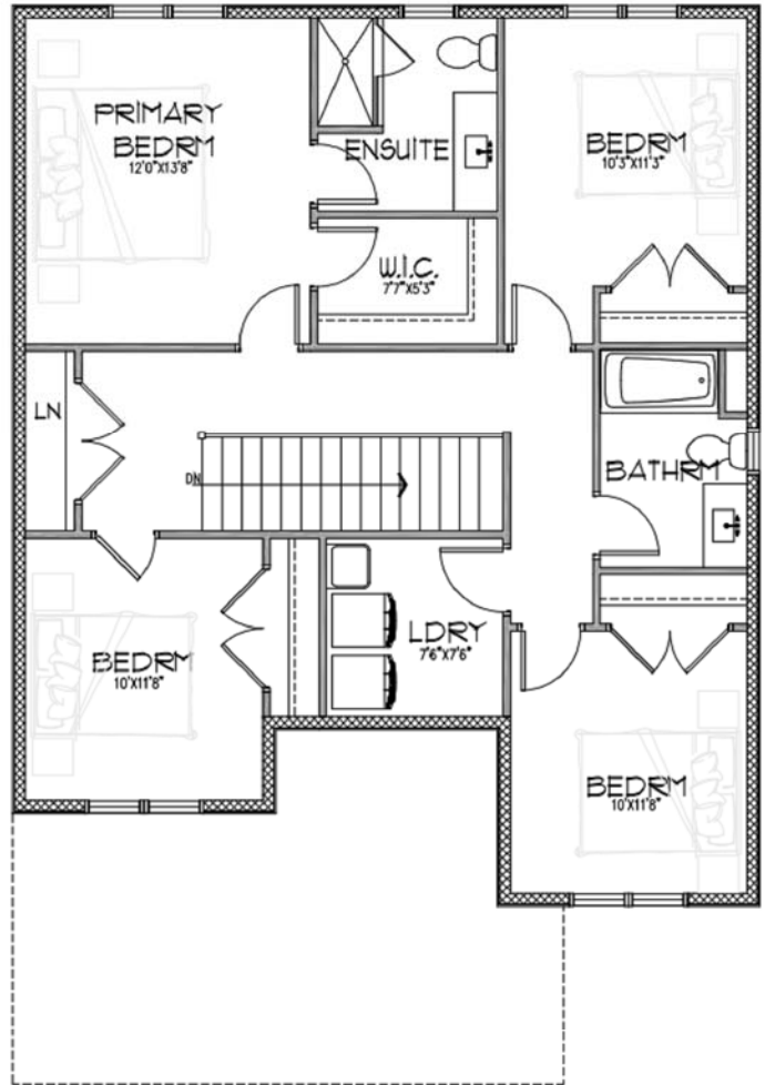
SECOND FLOOR 1082 SQFT
