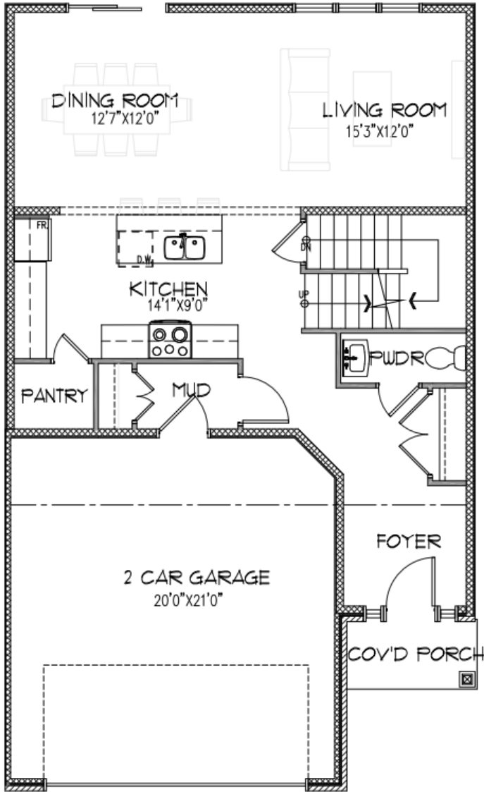
MAIN FLOOR 8116SQFT
