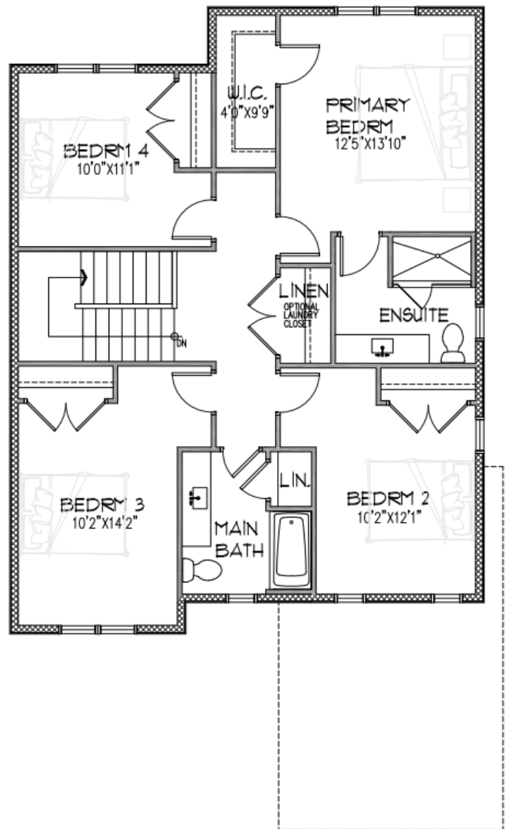
SECOND FLOOR 1126sqft
