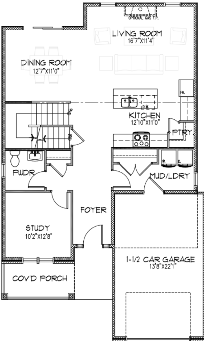
MAIN FLOOR 1024sqft
