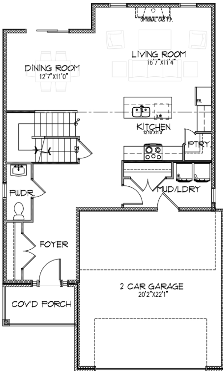
MAIN FLOOR 970sqft
